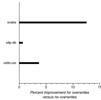
Fig. 10. Effect of allowing write cache overwrites on performance.
